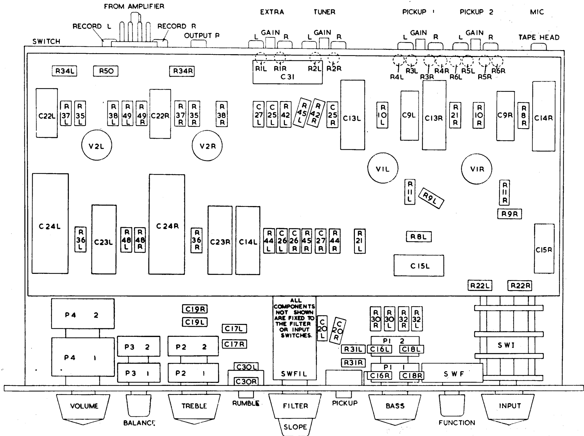
CHASSIS LAYOUT
